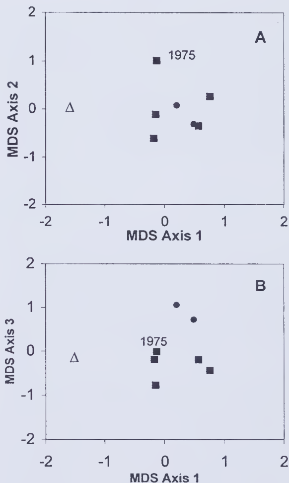
Figure 4. Three-dimensional ordination of 8 waterbird surveys from Toolibin Lake, based on species composition, showing relative positions of pre-salinization ( \Delta ), baseline (1975, 1981-84, \blacksquare ) and 1996 surveys ( \bullet ); stress = 0.10.
